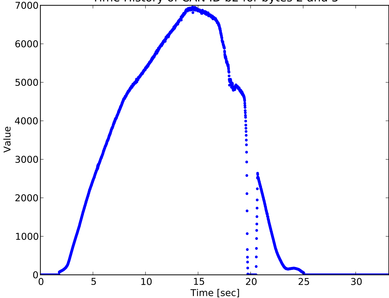
Time History of CAN ID b2 for bytes 2 and 3
