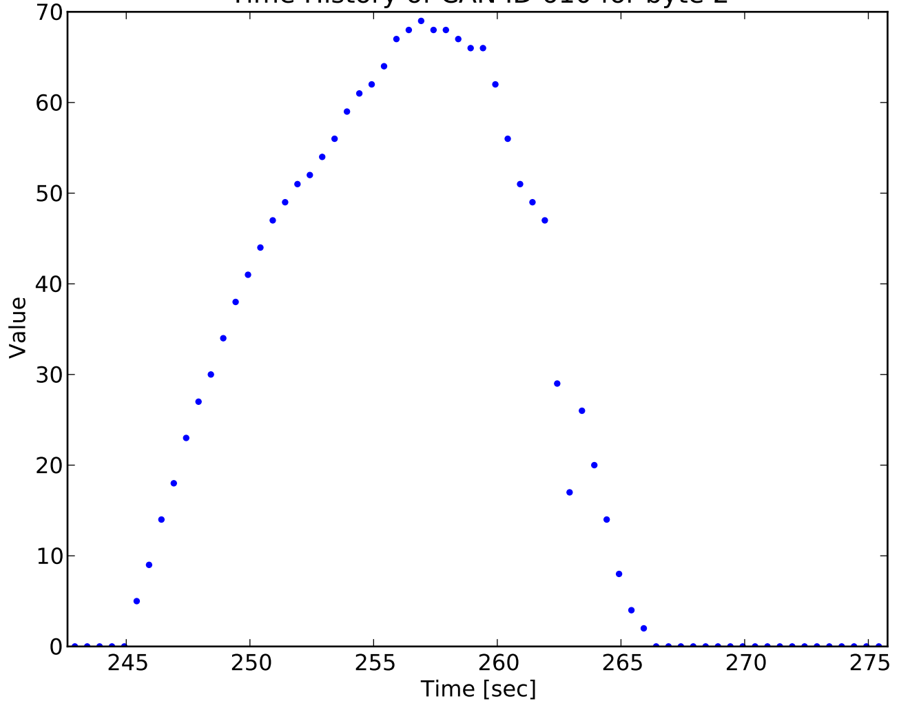
Time History of CAN ID 610 for byte 2
