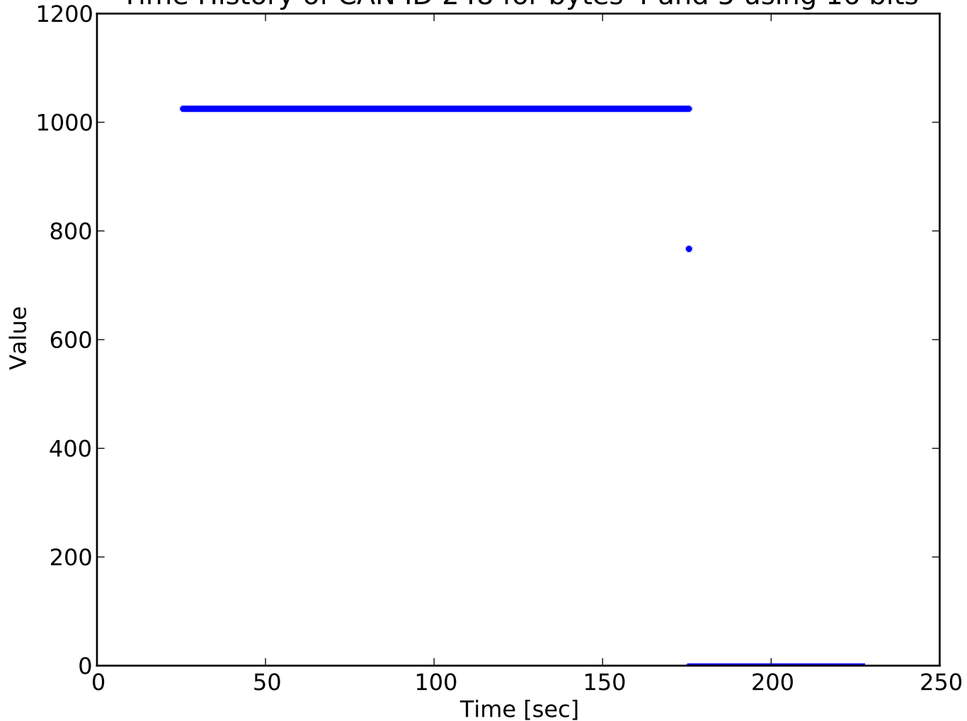
Time History of CAN ID 248 for bytes 4 and 5 using 16 bits
