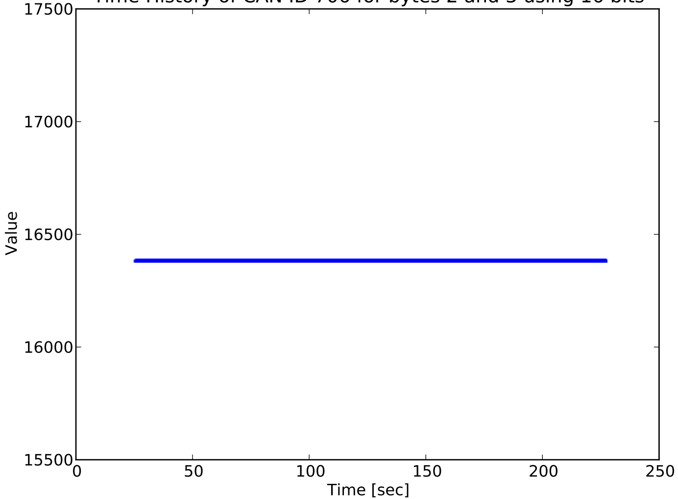
Time History of CAN ID 706 for bytes 2 and 3 using 16 bits
