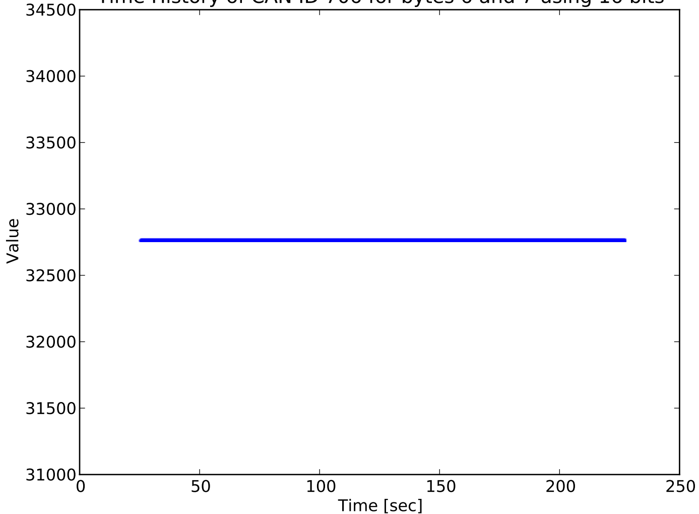
Time History of CAN ID 706 for bytes 6 and 7 using 16 bits
