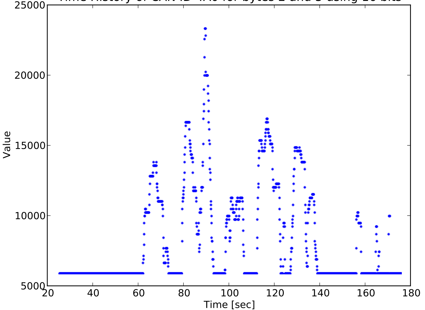
Time History of CAN ID 4A0 for bytes 2 and 3 using 16 bits
