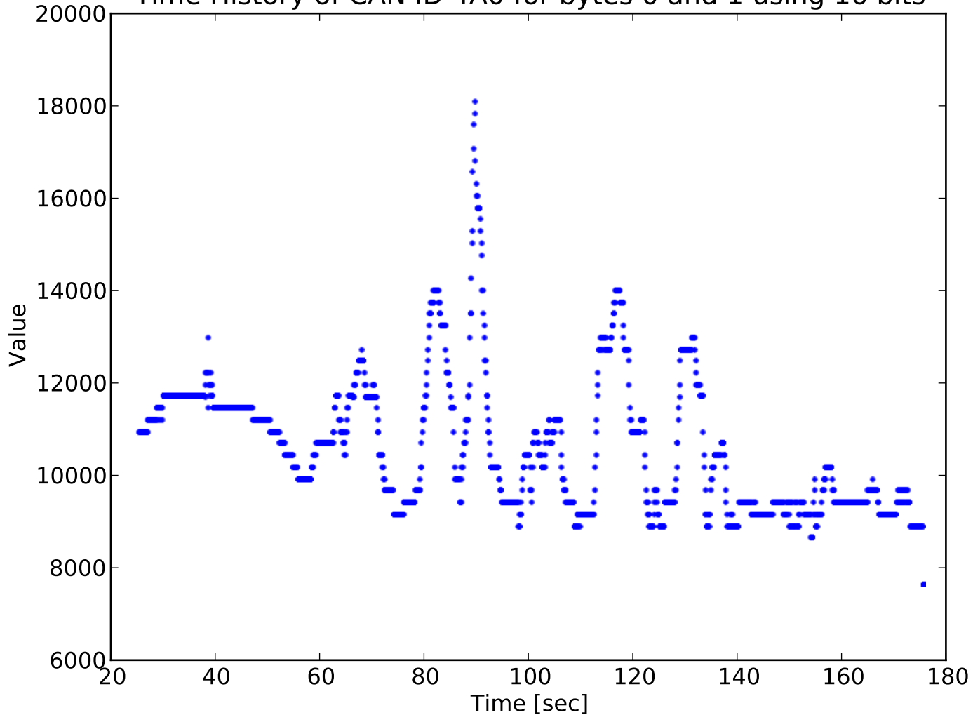
Time History of CAN ID 4A0 for bytes 0 and 1 using 16 bits
