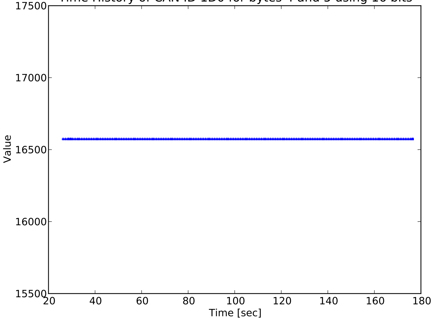
Time History of CAN ID 1D0 for bytes 4 and 5 using 16 bits
