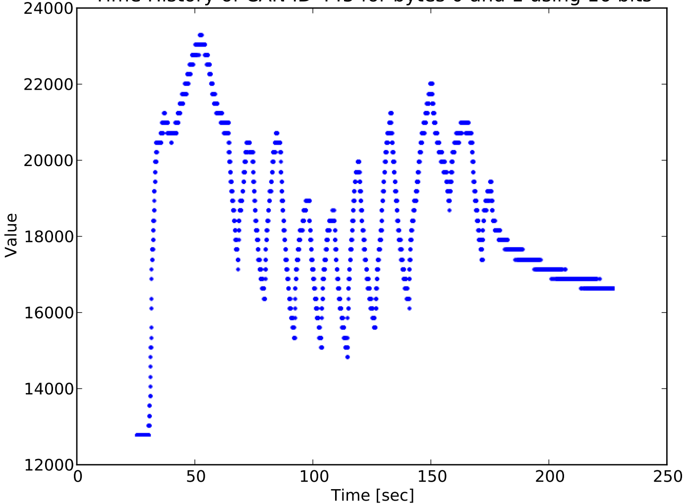
Time History of CAN ID 445 for bytes 0 and 1 using 16 bits
