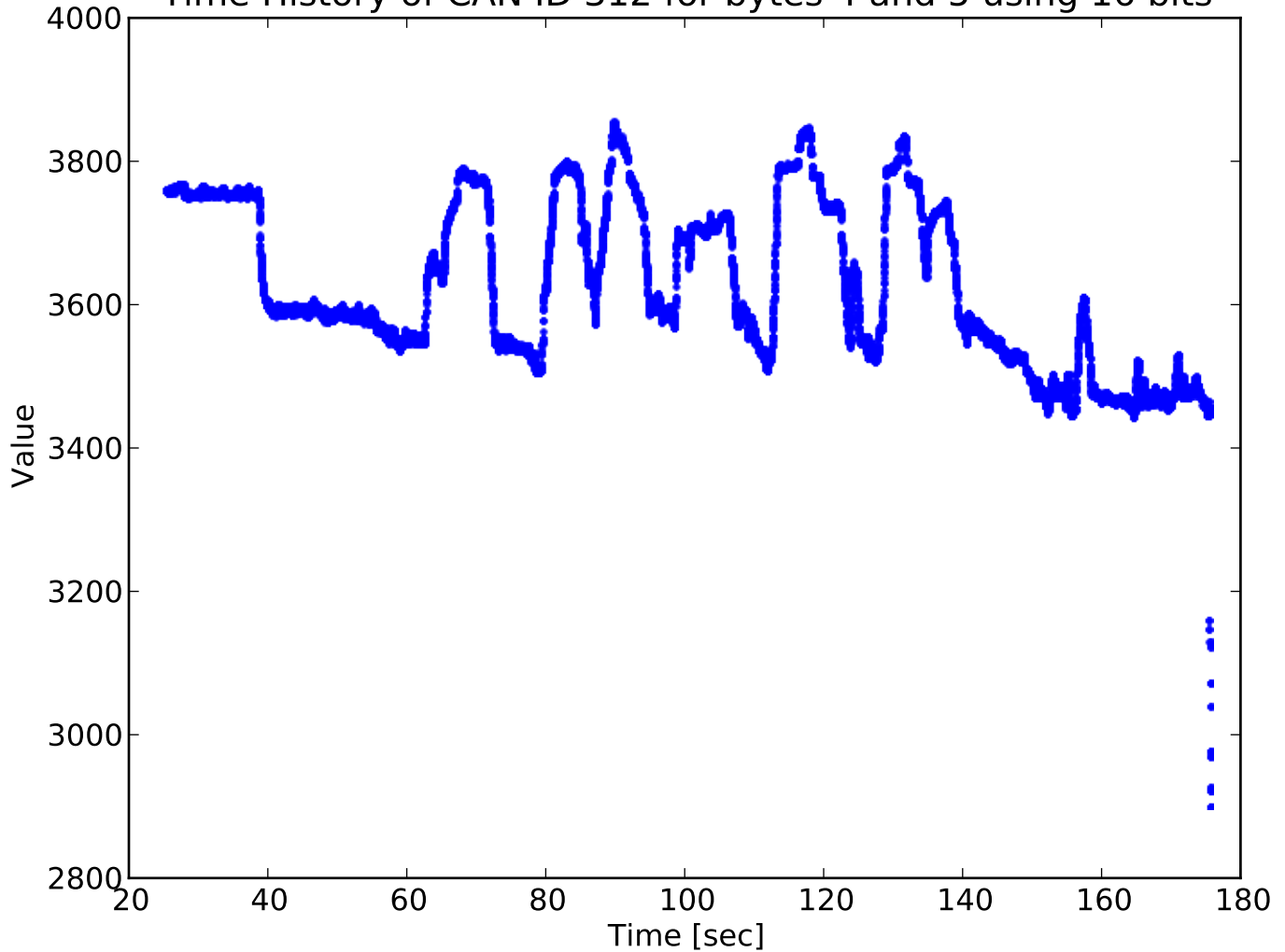
Time History of CAN ID 312 for bytes 4 and 5 using 16 bits
