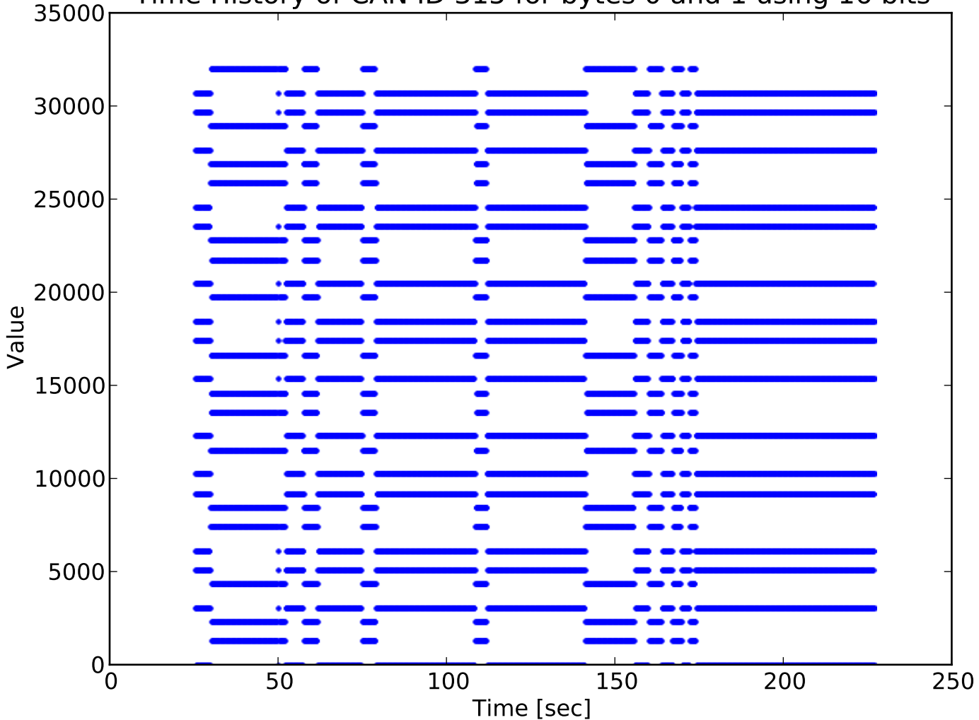
Time History of CAN ID 315 for bytes 0 and 1 using 16 bits
