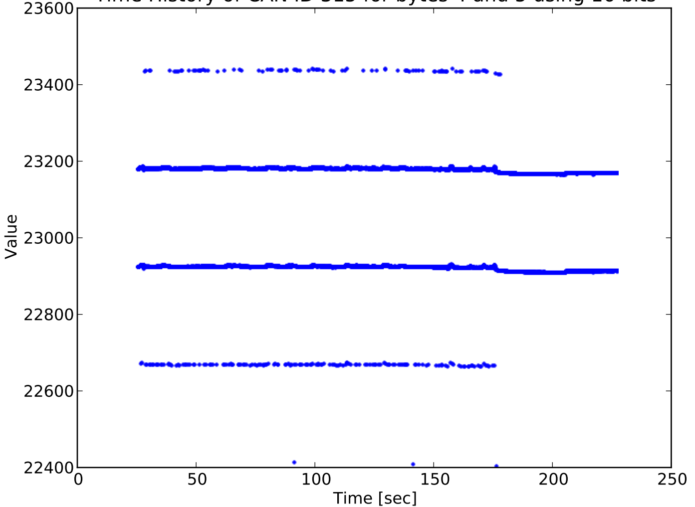
Time History of CAN ID 315 for bytes 4 and 5 using 16 bits
