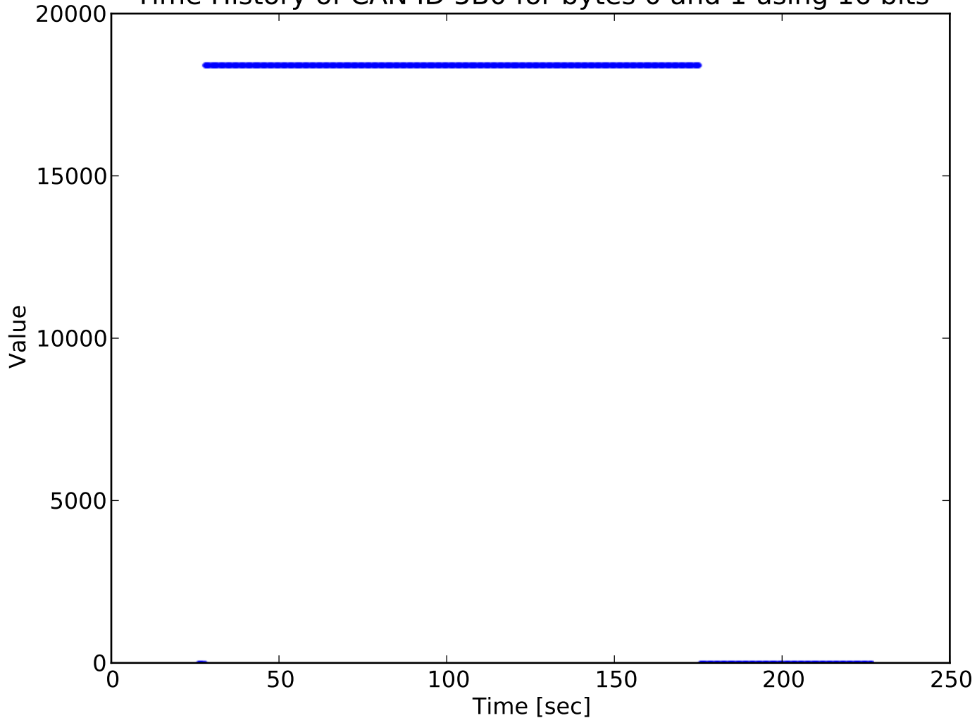
Time History of CAN ID 5B0 for bytes 0 and 1 using 16 bits
