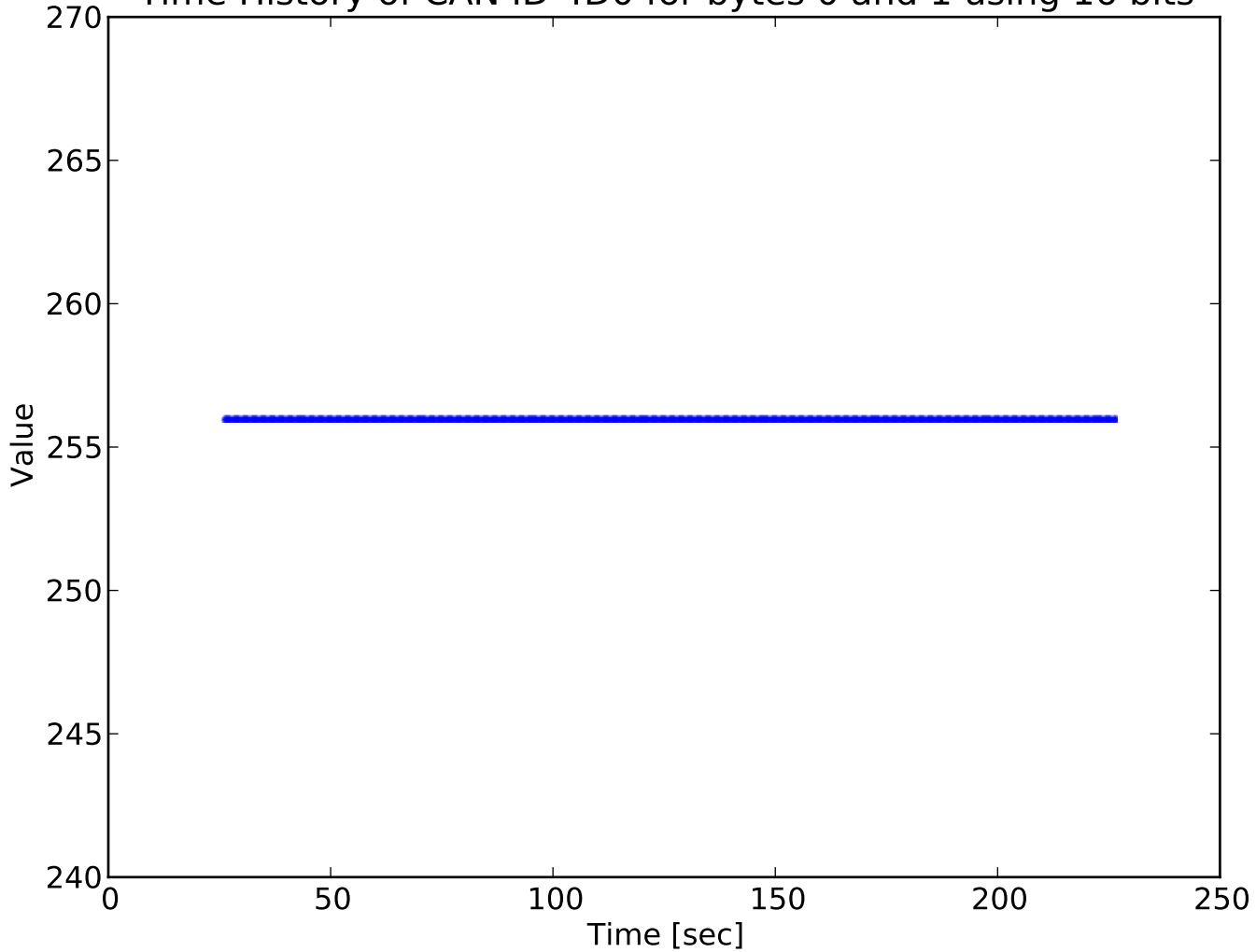
Time History of CAN ID 4D0 for bytes 0 and 1 using 16 bits
