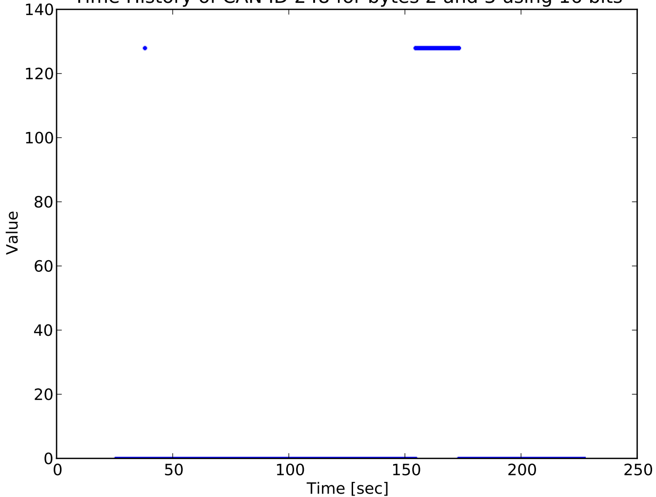
Time History of CAN ID 248 for bytes 2 and 3 using 16 bits
