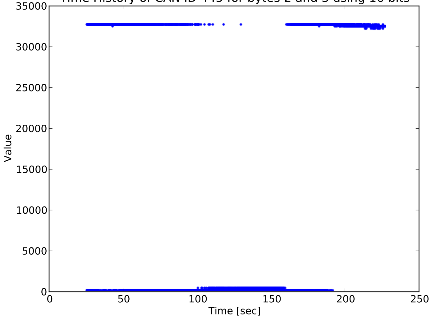
Time History of CAN ID 445 for bytes 2 and 3 using 16 bits
