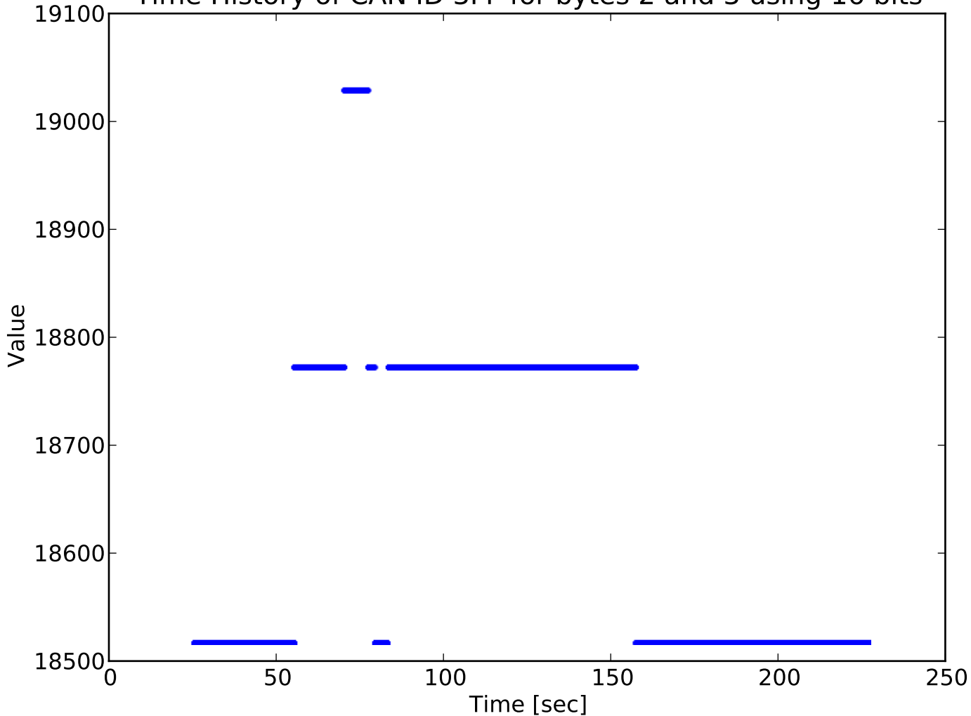
Time History of CAN ID 3FF for bytes 2 and 3 using 16 bits
