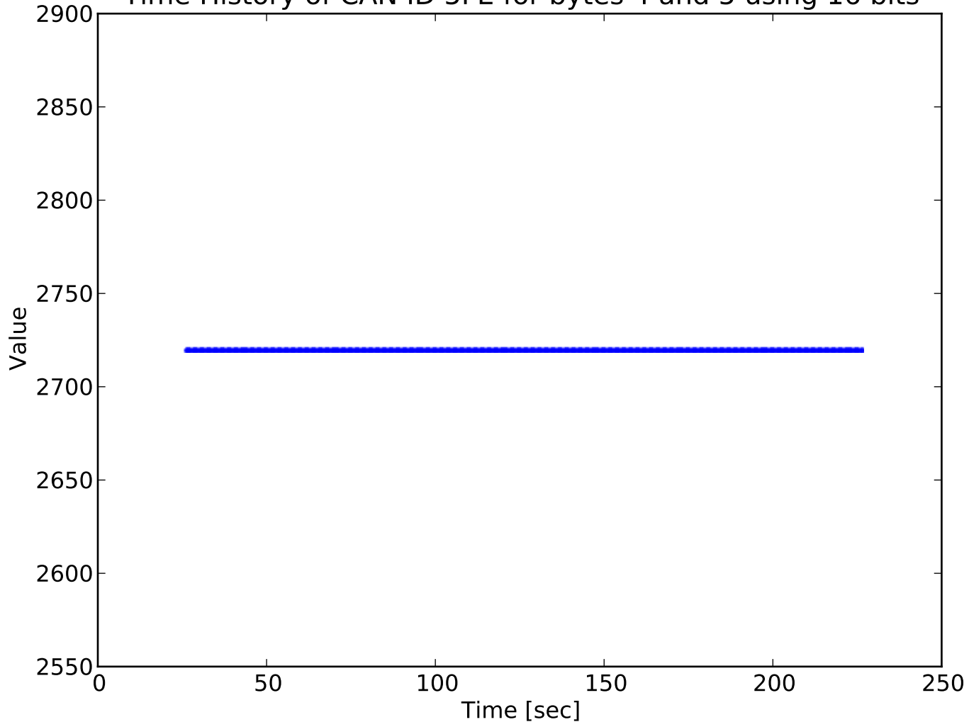
Time History of CAN ID 5FE for bytes 4 and 5 using 16 bits
