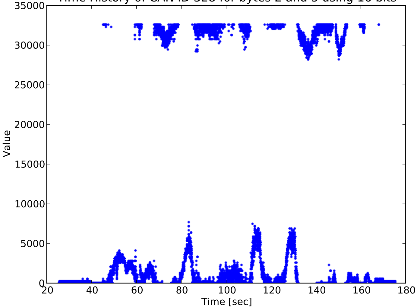
Time History of CAN ID 328 for bytes 2 and 3 using 16 bits
