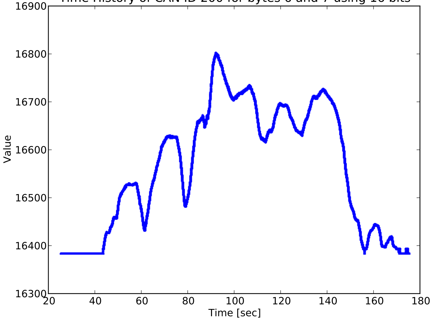
Time History of CAN ID 200 for bytes 6 and 7 using 16 bits
