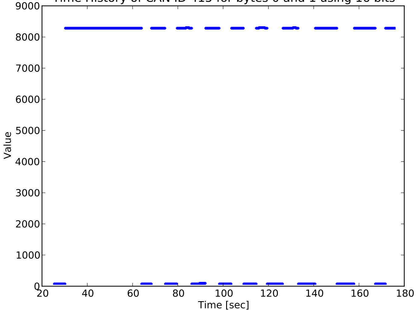
Time History of CAN ID 415 for bytes 0 and 1 using 16 bits
