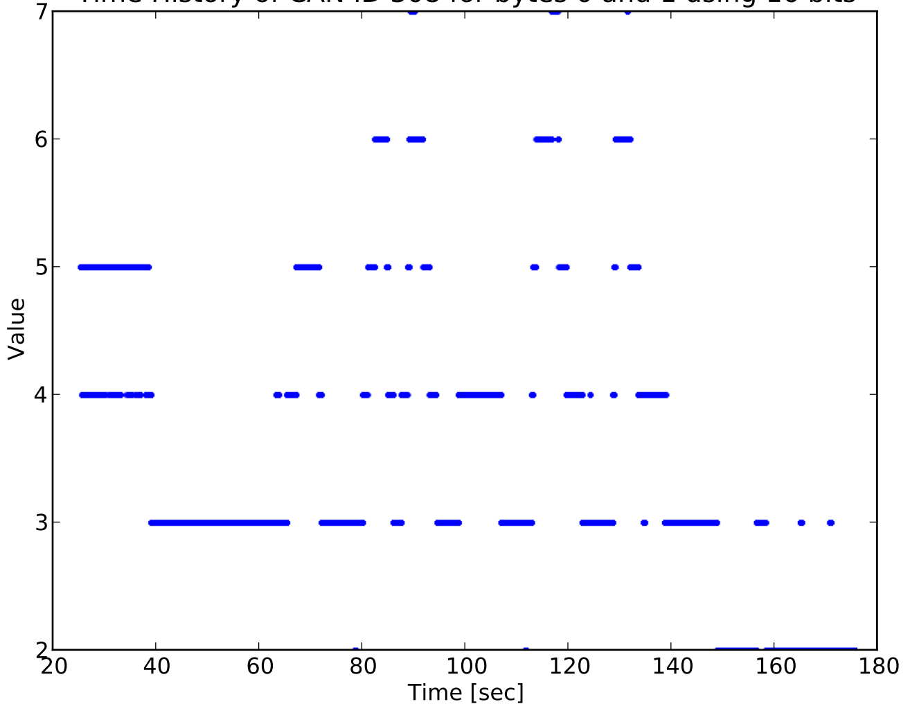
Time History of CAN ID 308 for bytes 0 and 1 using 16 bits
