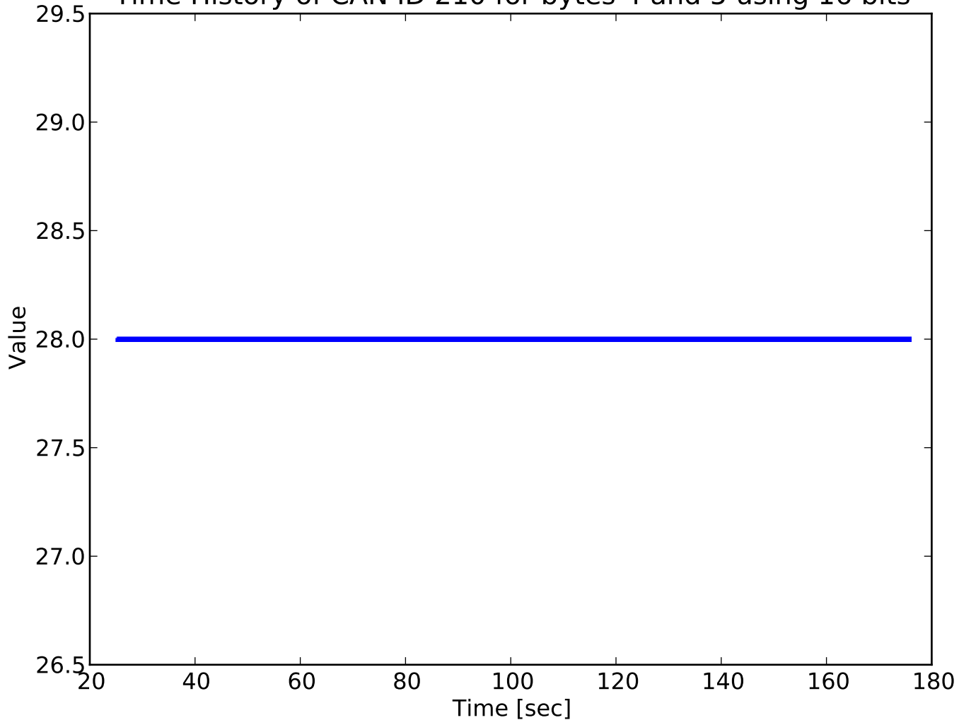
Time History of CAN ID 210 for bytes 4 and 5 using 16 bits
