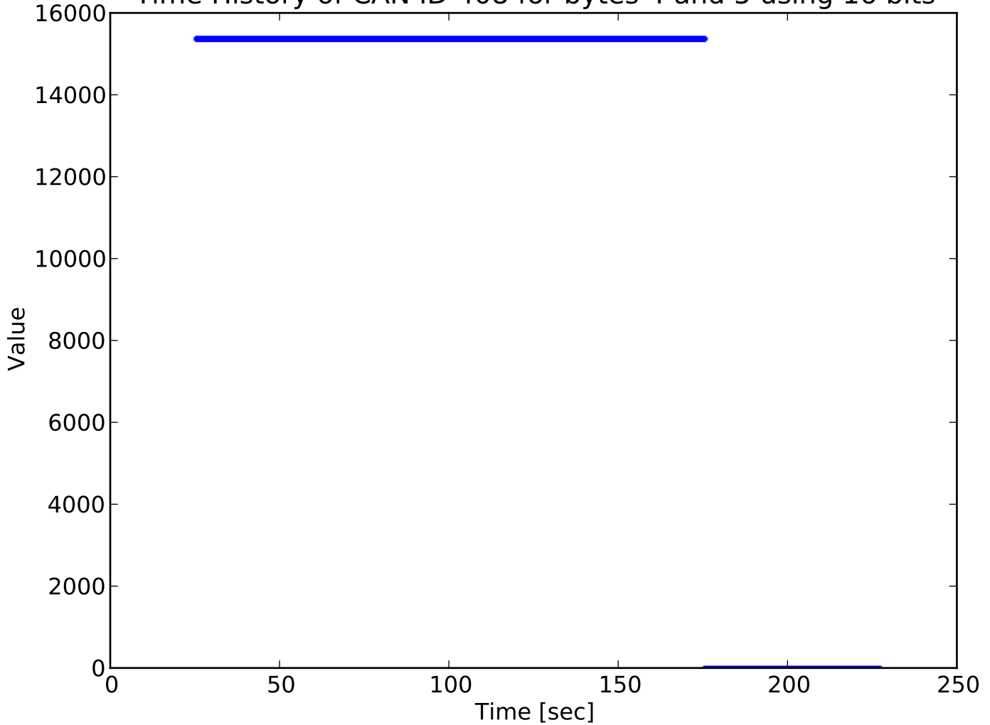
Time History of CAN ID 408 for bytes 4 and 5 using 16 bits
