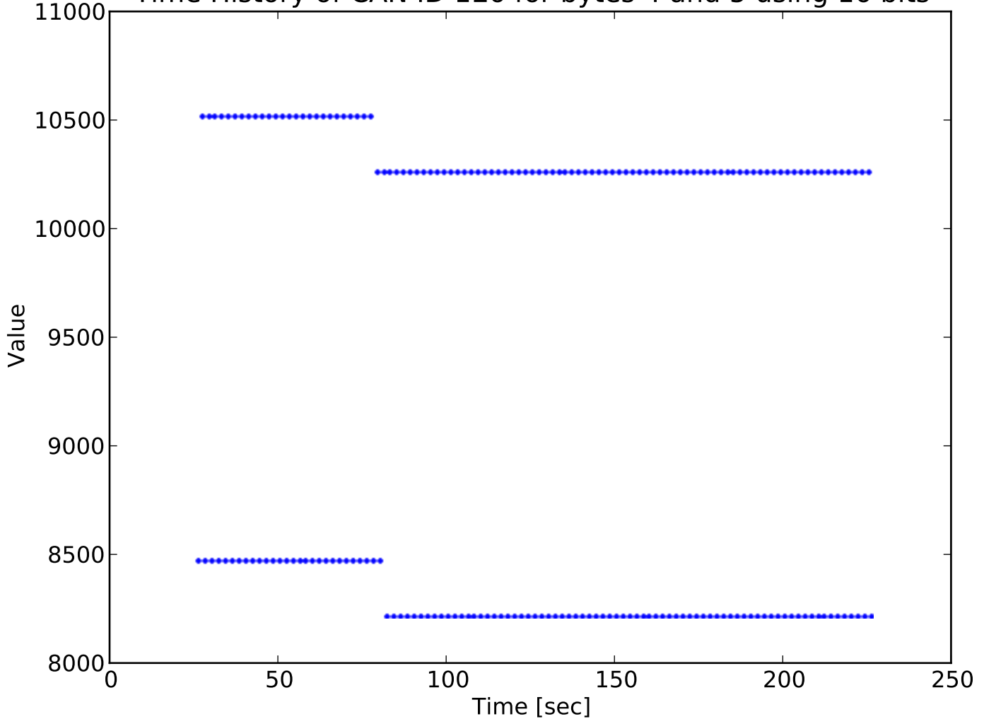
Time History of CAN ID 1E6 for bytes 4 and 5 using 16 bits
