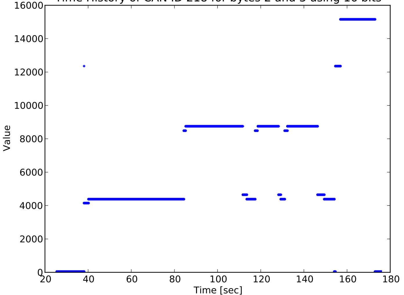
Time History of CAN ID 218 for bytes 2 and 3 using 16 bits
