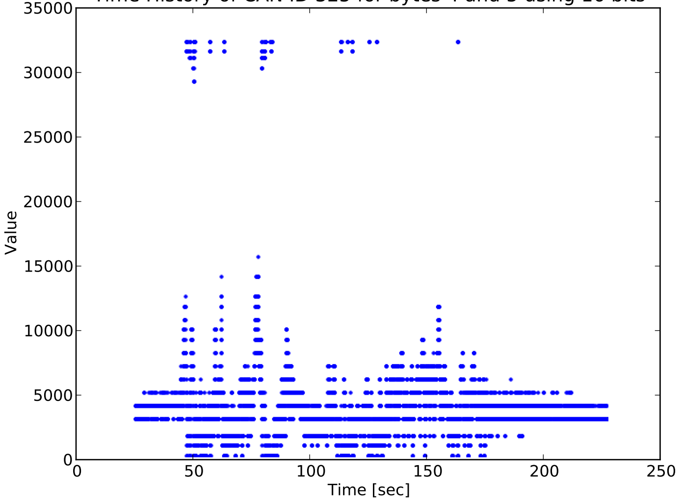
Time History of CAN ID 325 for bytes 4 and 5 using 16 bits
