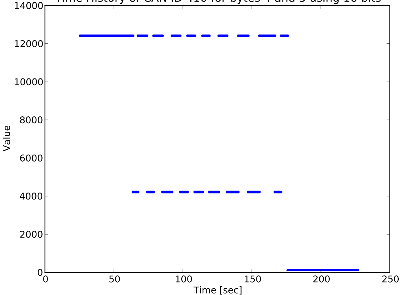
Time History of CAN ID 410 for bytes 4 and 5 using 16 bits
