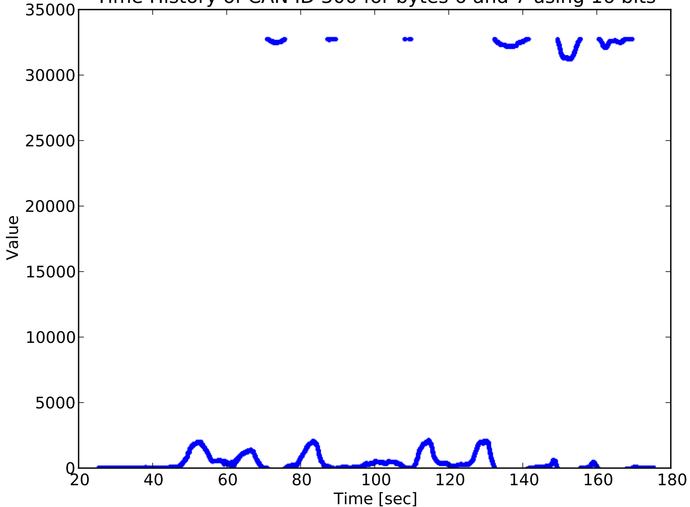
Time History of CAN ID 300 for bytes 6 and 7 using 16 bits
