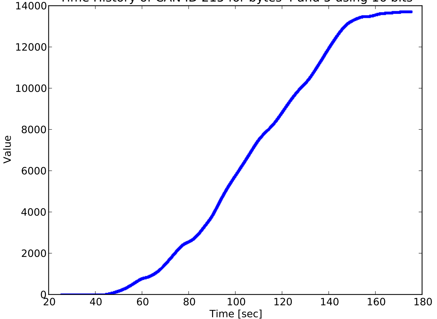
Time History of CAN ID 215 for bytes 4 and 5 using 16 bits
