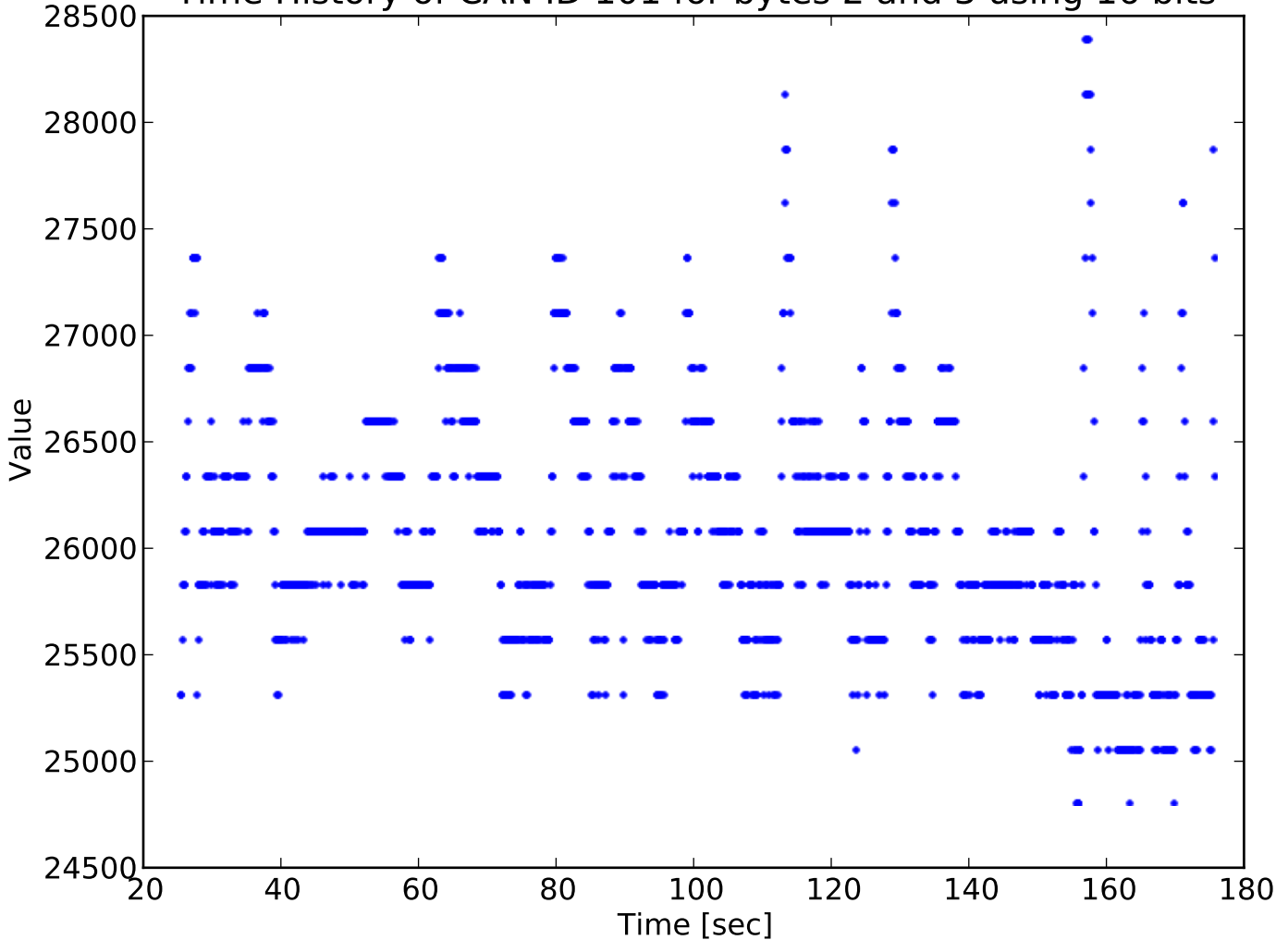
Time History of CAN ID 101 for bytes 2 and 3 using 16 bits
