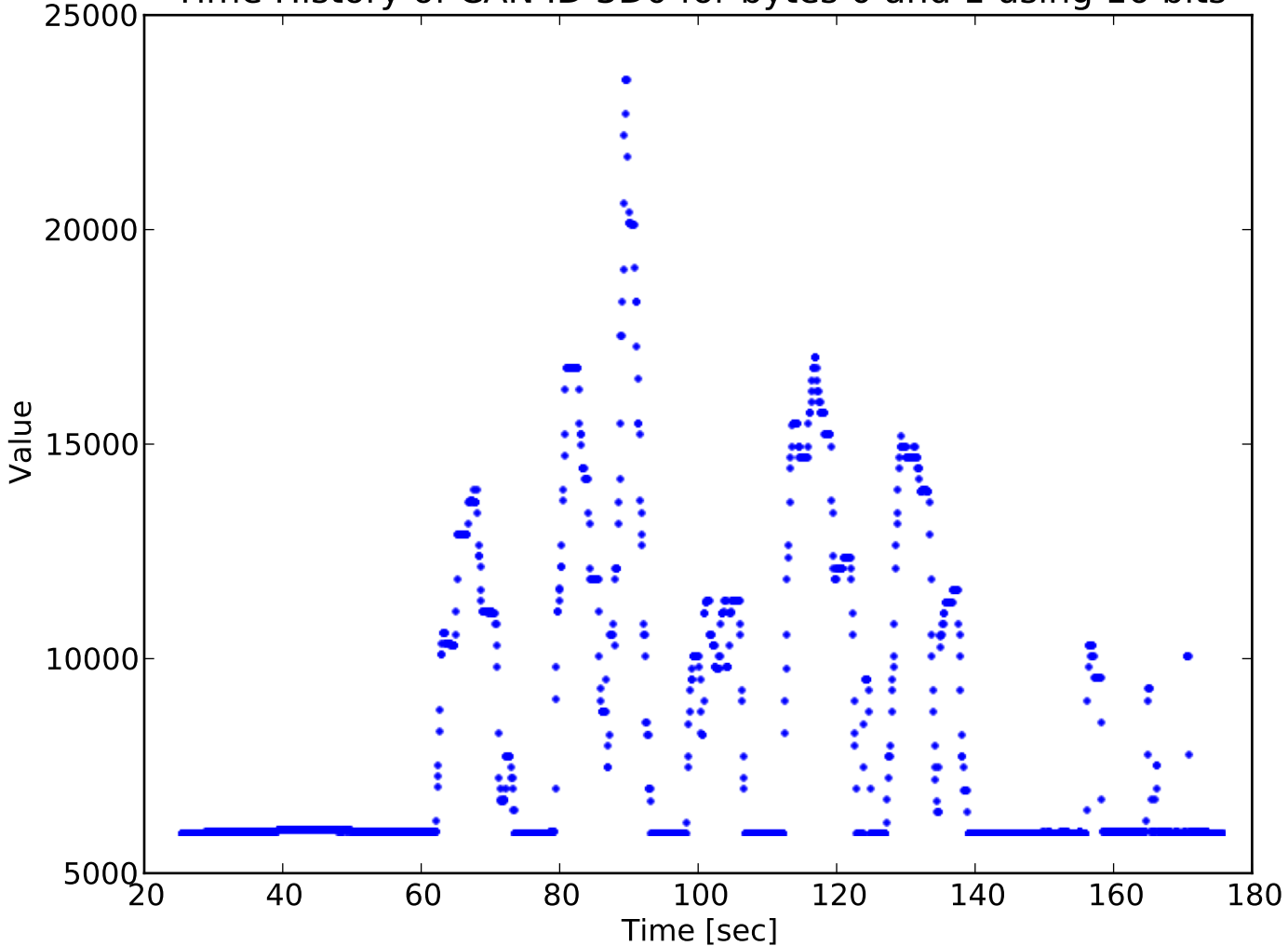
Time History of CAN ID 3D0 for bytes 0 and 1 using 16 bits
