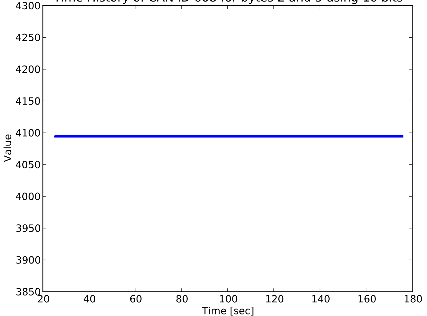
Time History of CAN ID 608 for bytes 2 and 3 using 16 bits
