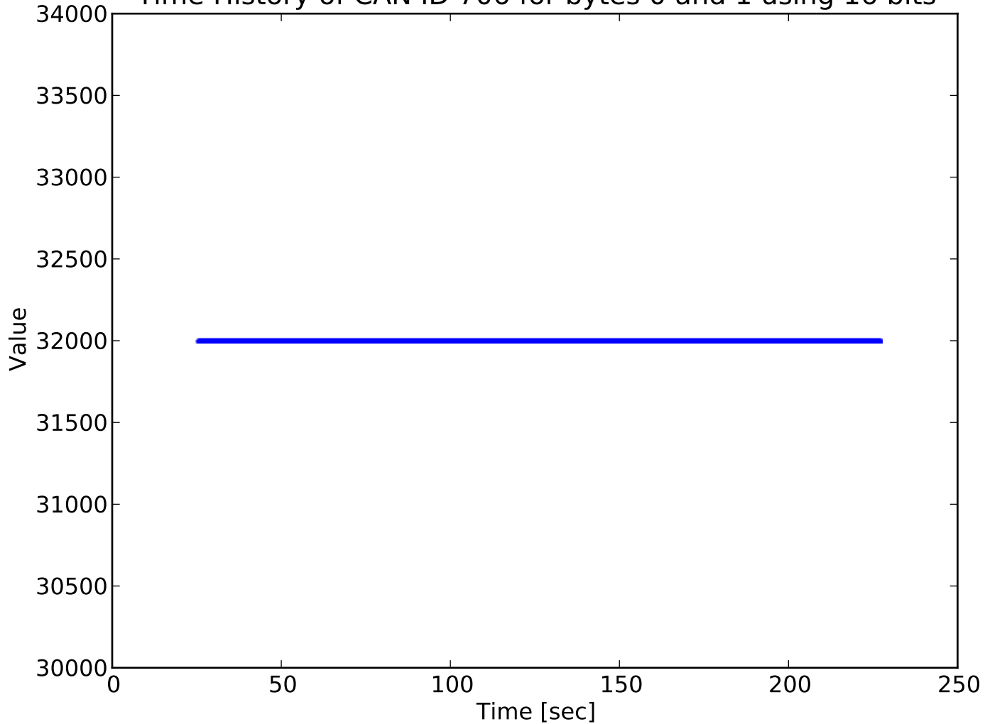
Time History of CAN ID 706 for bytes 0 and 1 using 16 bits
