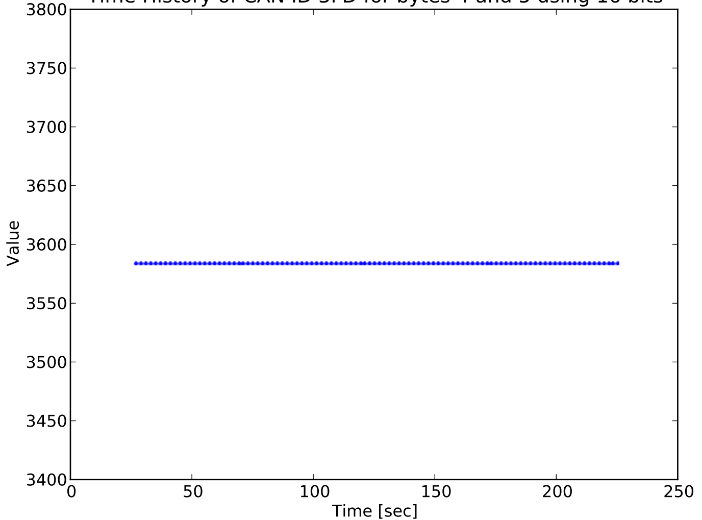
Time History of CAN ID 3FD for bytes 4 and 5 using 16 bits
