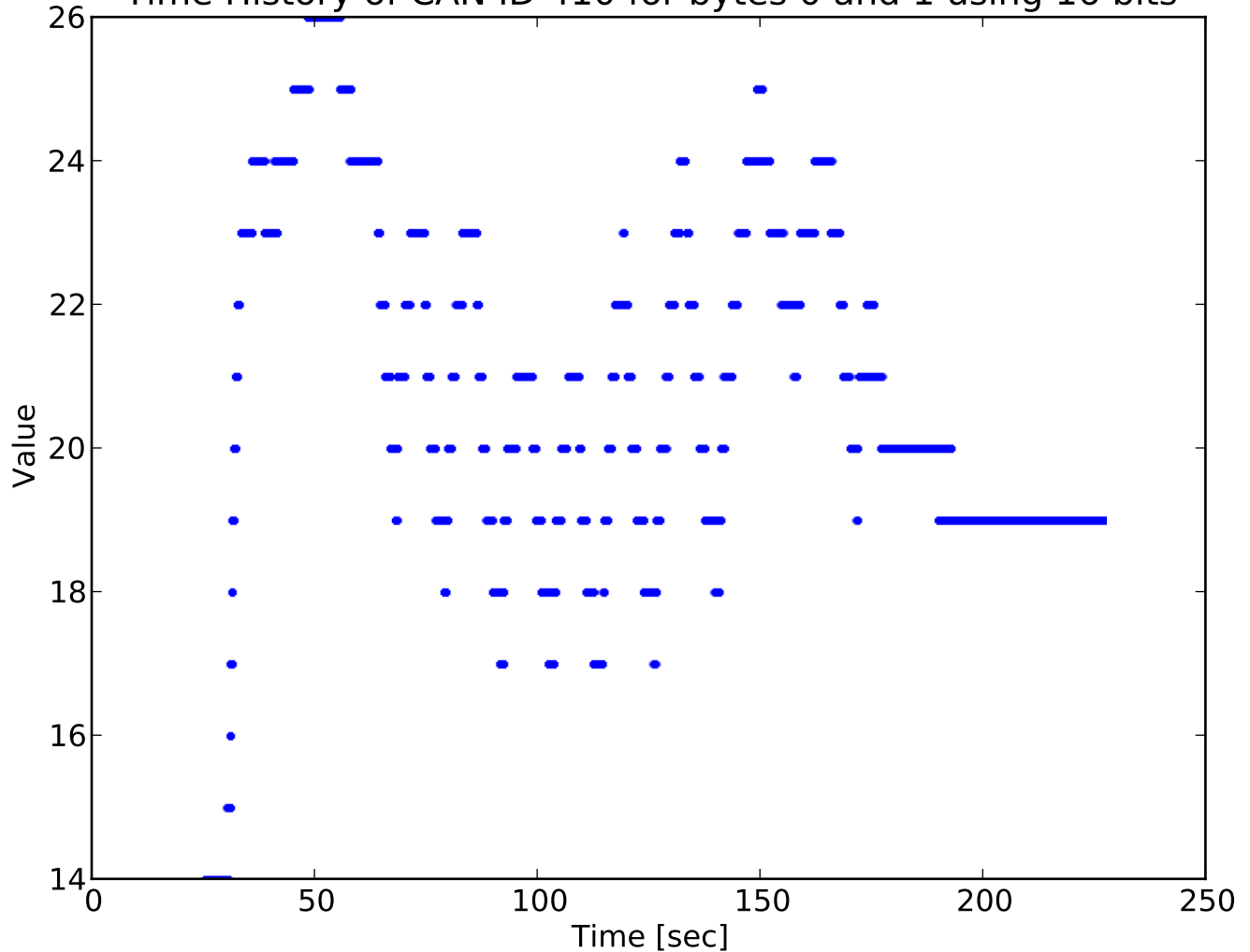
Time History of CAN ID 410 for bytes 0 and 1 using 16 bits
