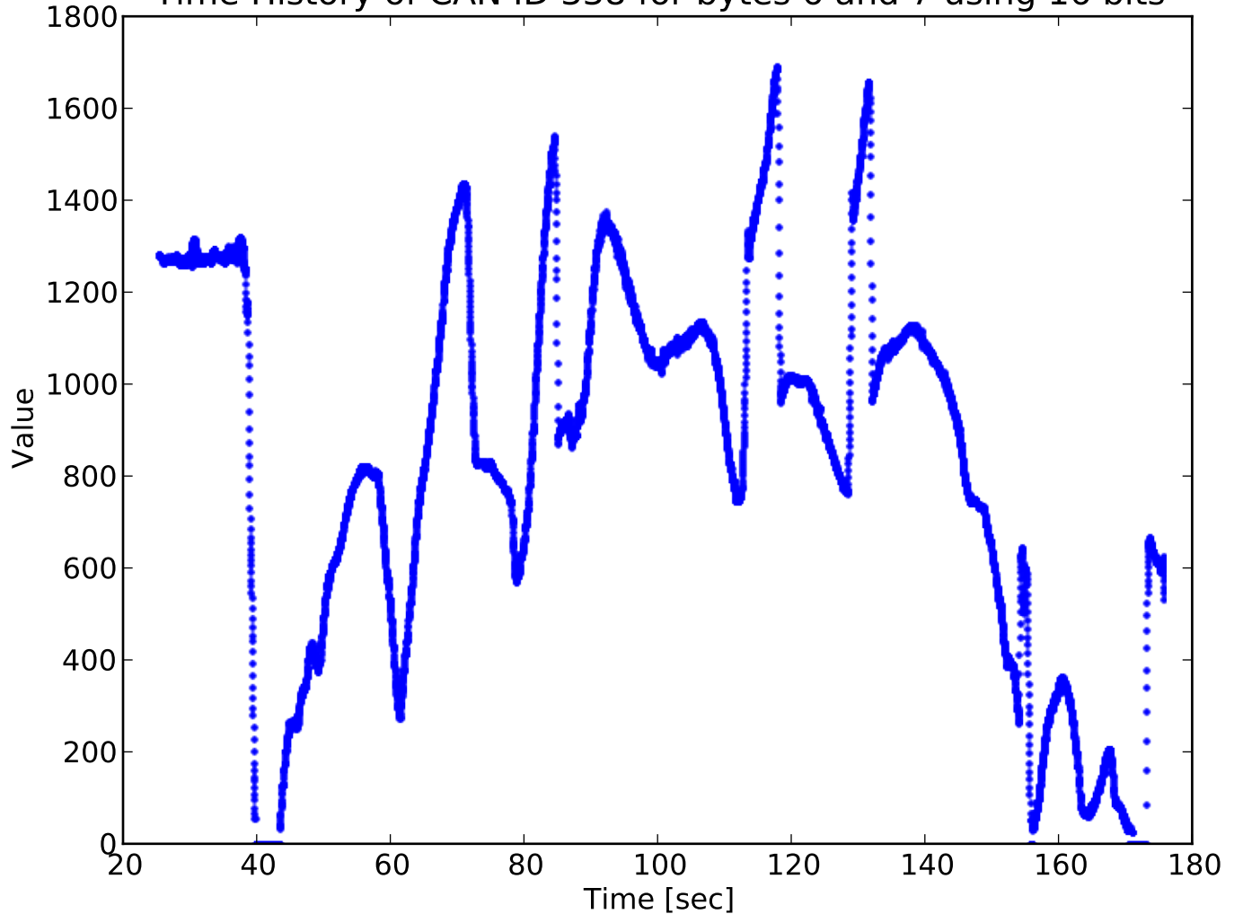
Time History of CAN ID 338 for bytes 6 and 7 using 16 bits
