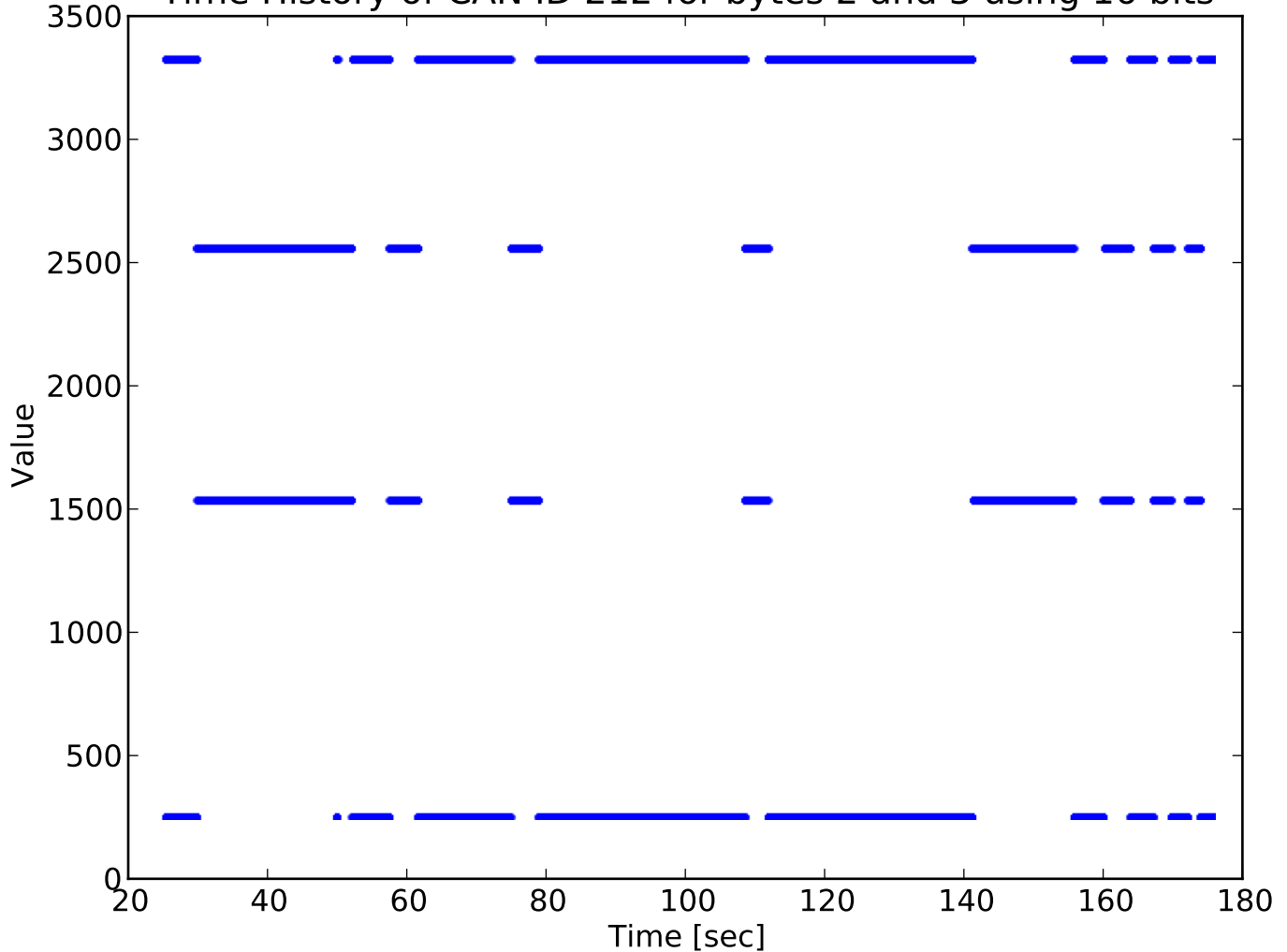
Time History of CAN ID 212 for bytes 2 and 3 using 16 bits
