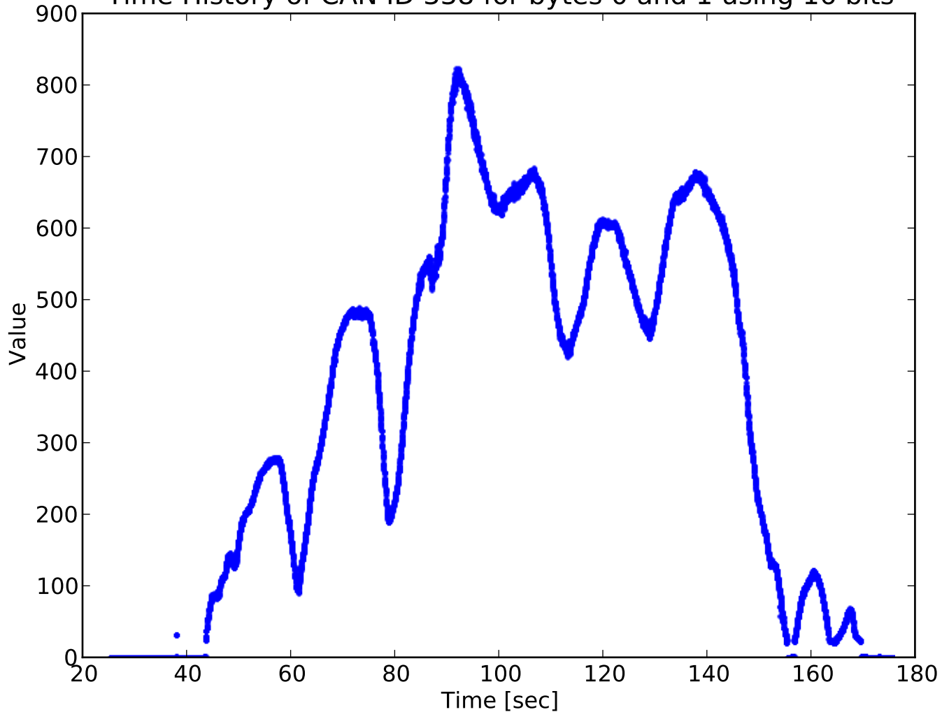
Time History of CAN ID 338 for bytes 0 and 1 using 16 bits
