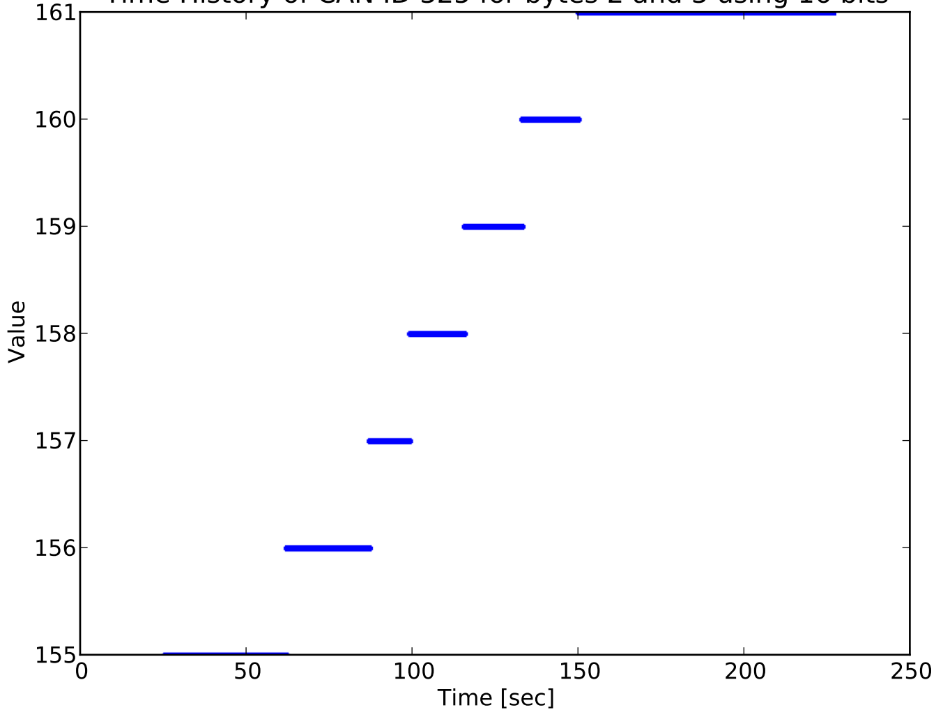
Time History of CAN ID 325 for bytes 2 and 3 using 16 bits
