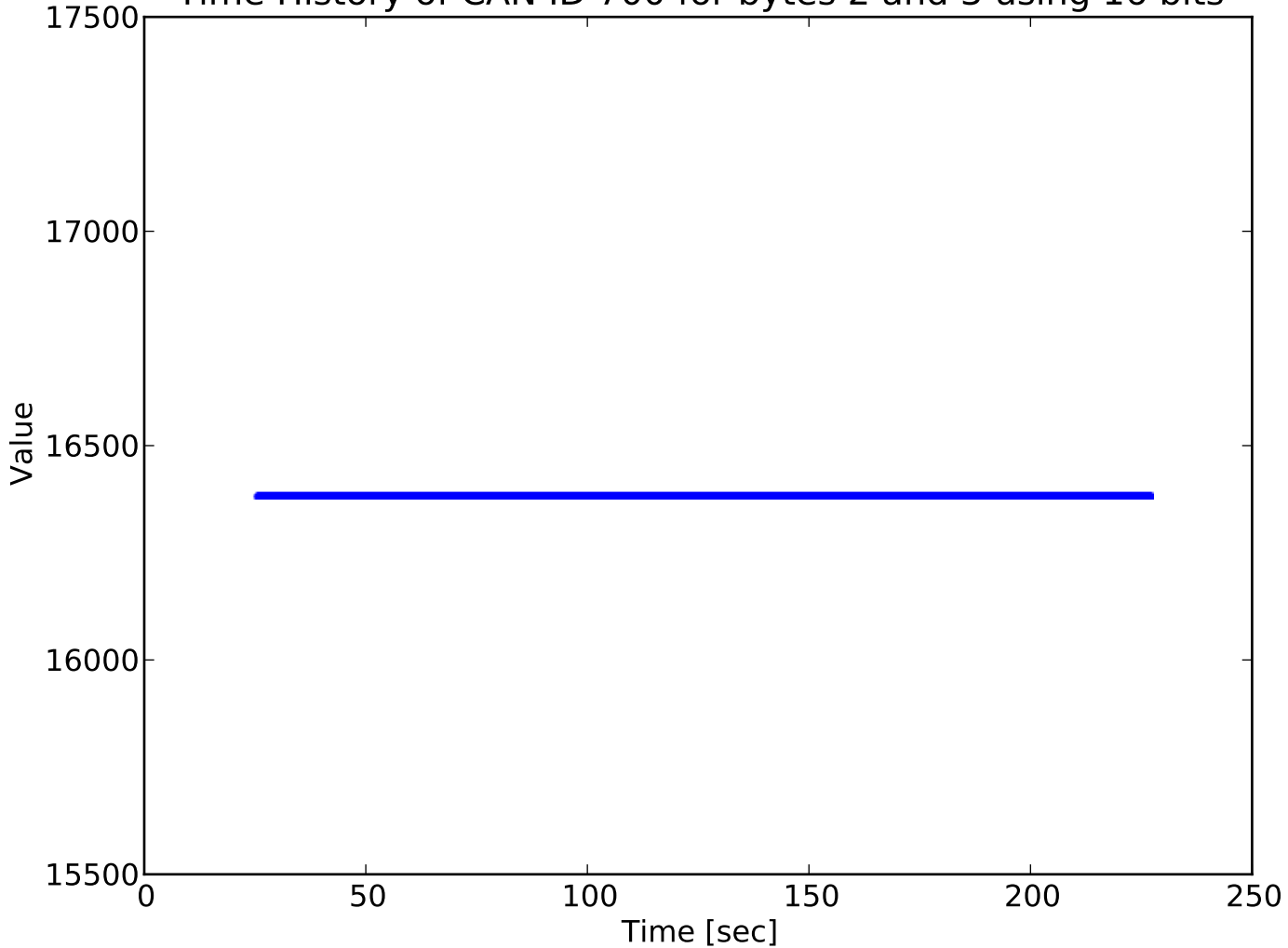
Time History of CAN ID 700 for bytes 2 and 3 using 16 bits
