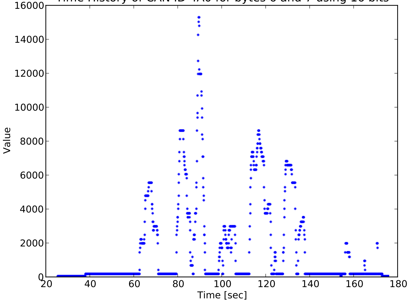
Time History of CAN ID 4A0 for bytes 6 and 7 using 16 bits
