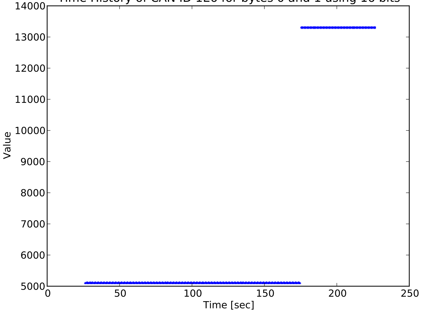
Time History of CAN ID 1E6 for bytes 0 and 1 using 16 bits
