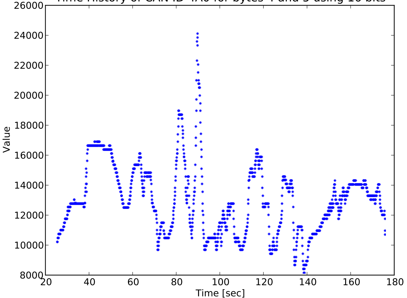
Time History of CAN ID 4A0 for bytes 4 and 5 using 16 bits
