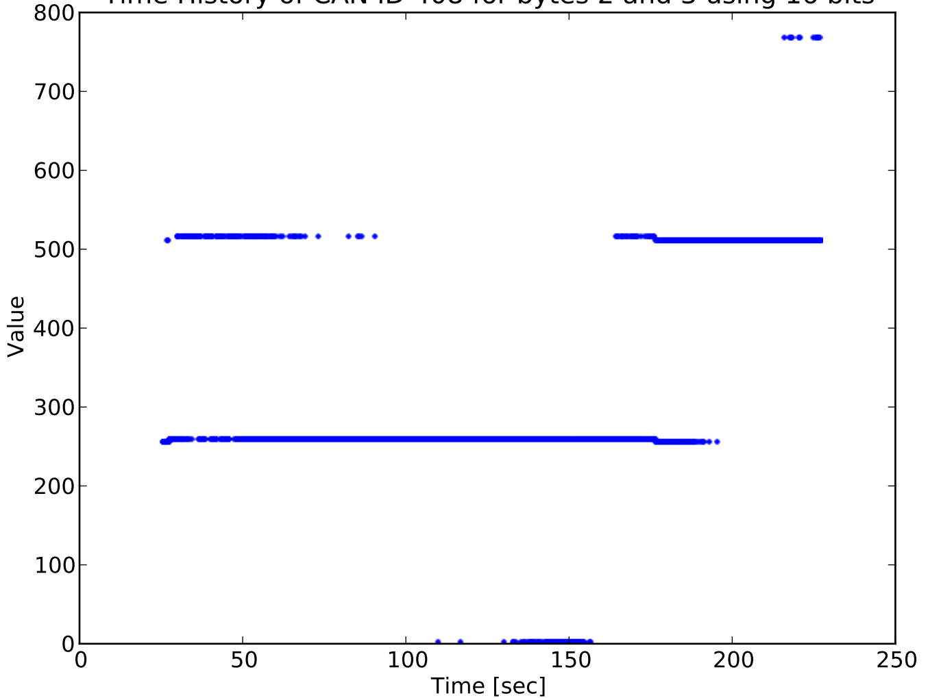
Time History of CAN ID 408 for bytes 2 and 3 using 16 bits
