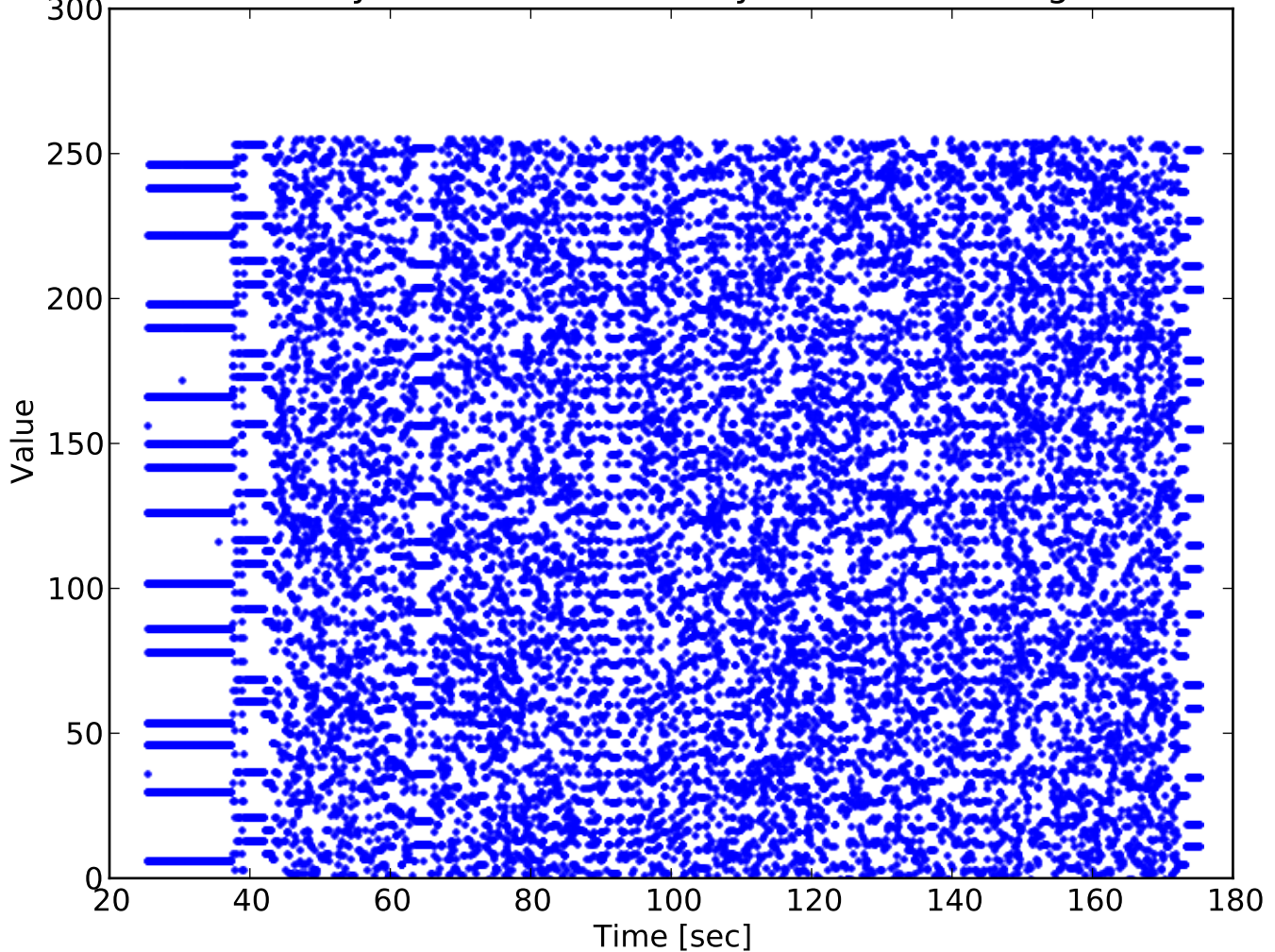
Time History of CAN ID 236 for bytes 6 and 7 using 16 bits
