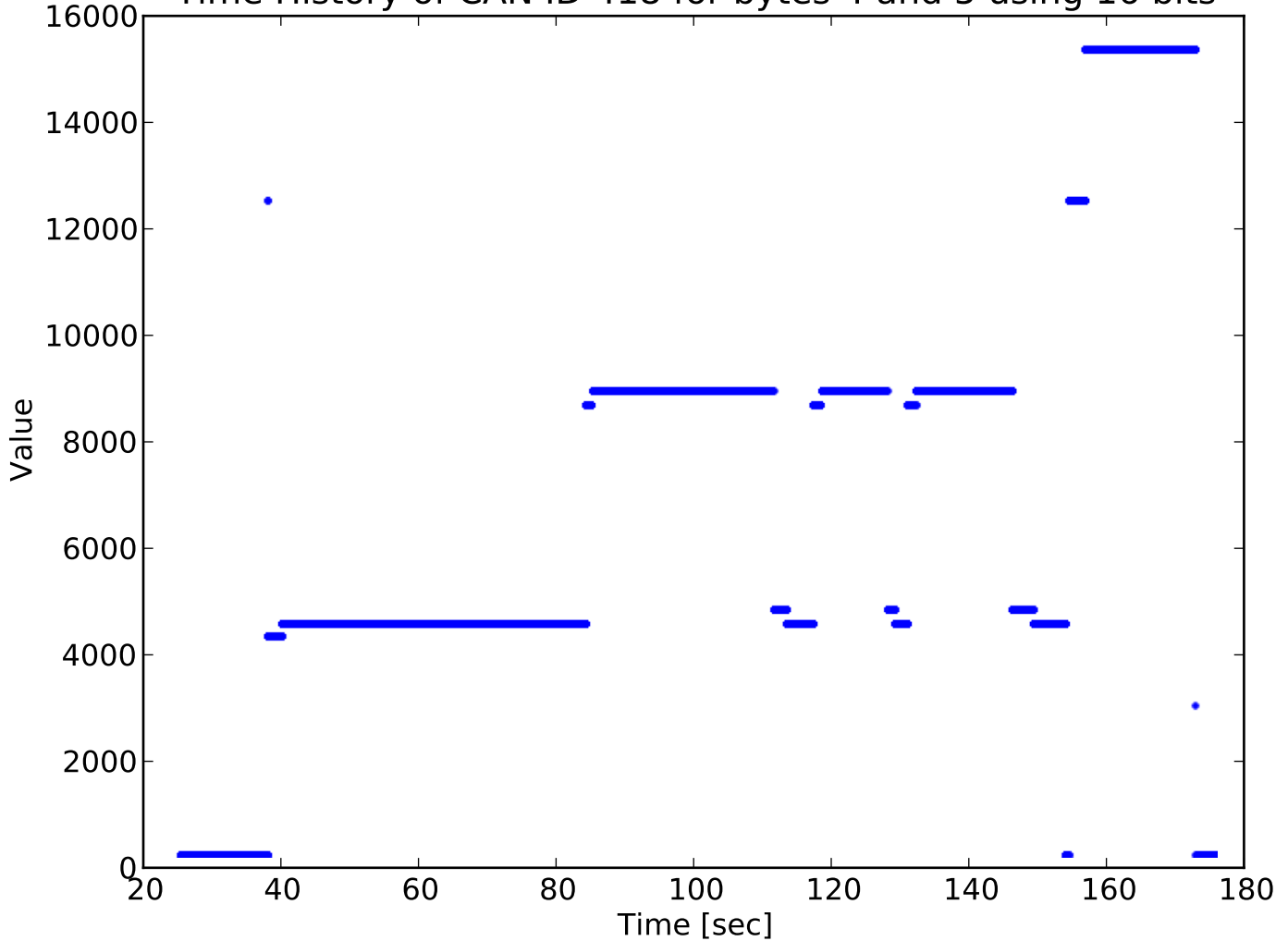
Time History of CAN ID 418 for bytes 4 and 5 using 16 bits
