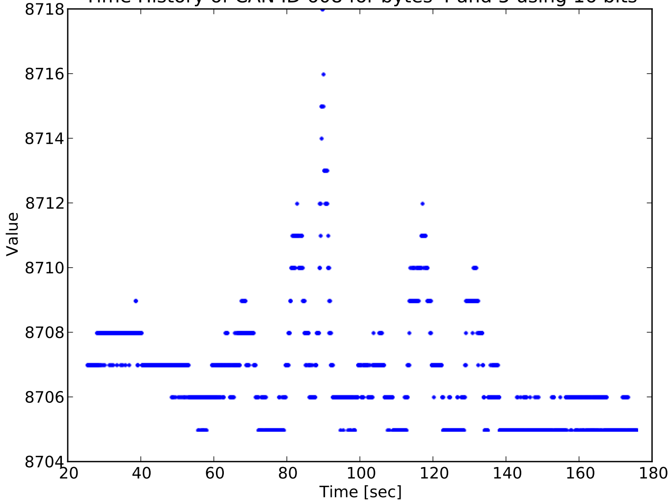
Time History of CAN ID 608 for bytes 4 and 5 using 16 bits
