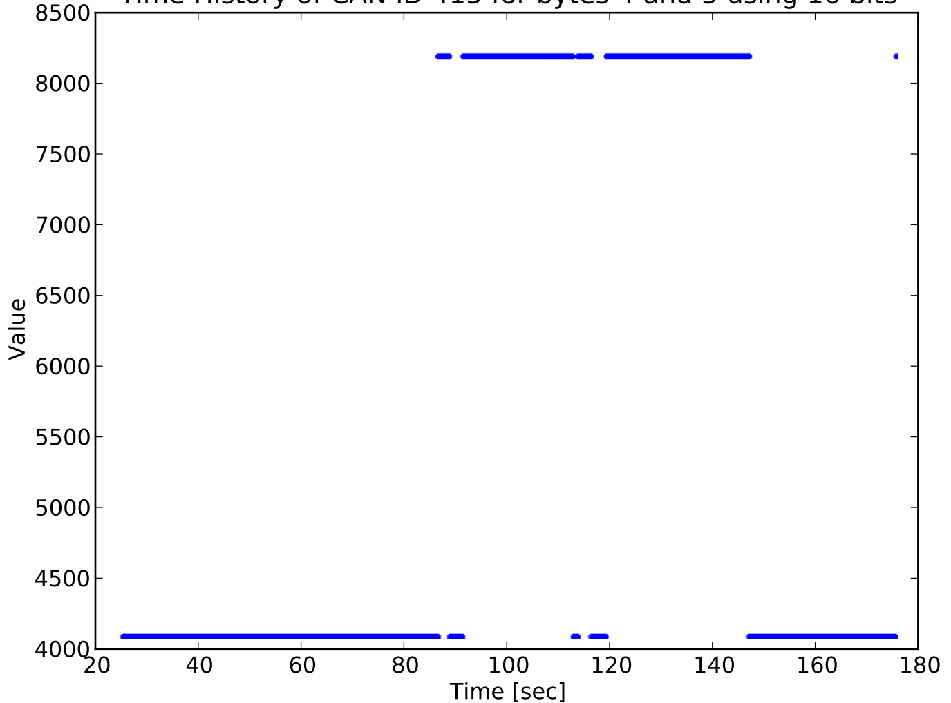
Time History of CAN ID 415 for bytes 4 and 5 using 16 bits
