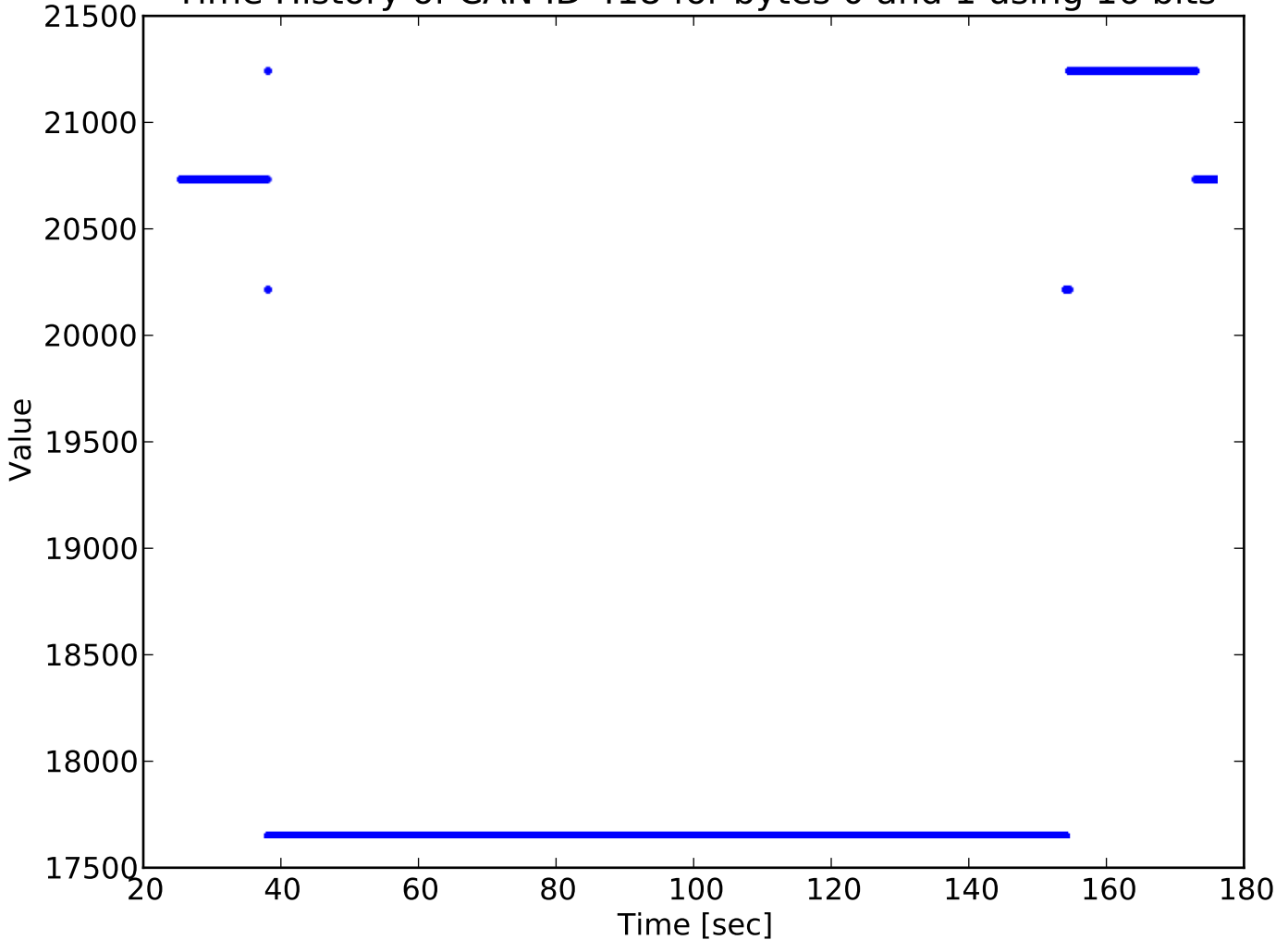
Time History of CAN ID 418 for bytes 0 and 1 using 16 bits
