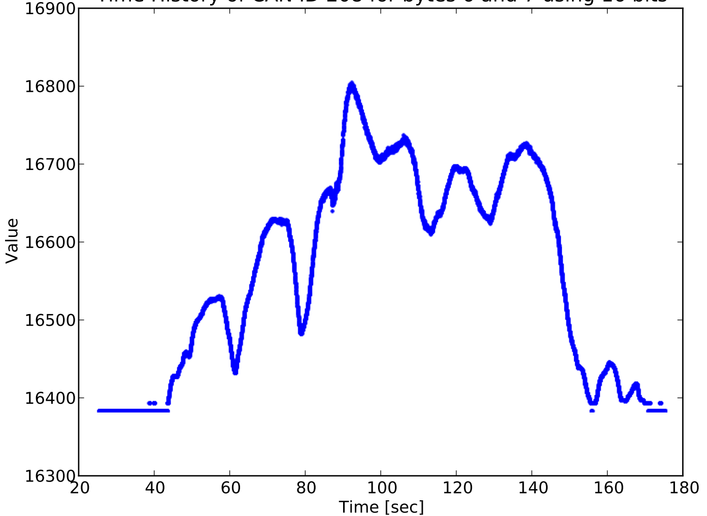
Time History of CAN ID 208 for bytes 6 and 7 using 16 bits
