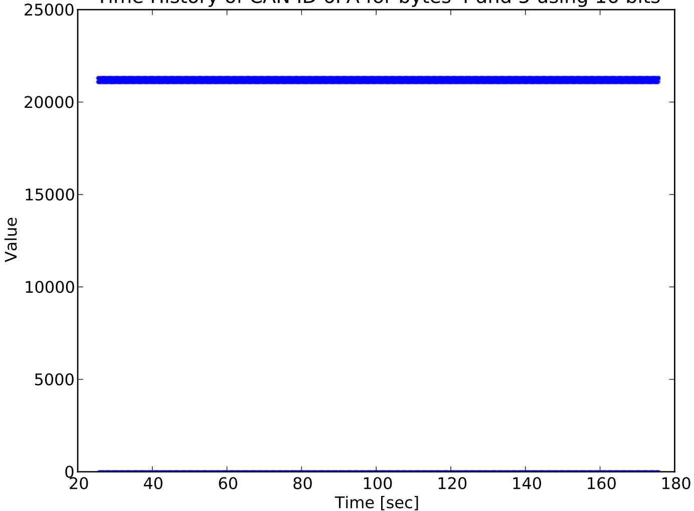
Time History of CAN ID 6FA for bytes 4 and 5 using 16 bits
