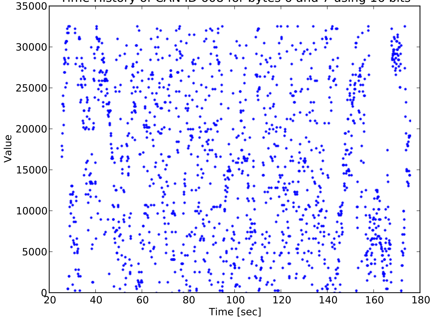
Time History of CAN ID 608 for bytes 6 and 7 using 16 bits
