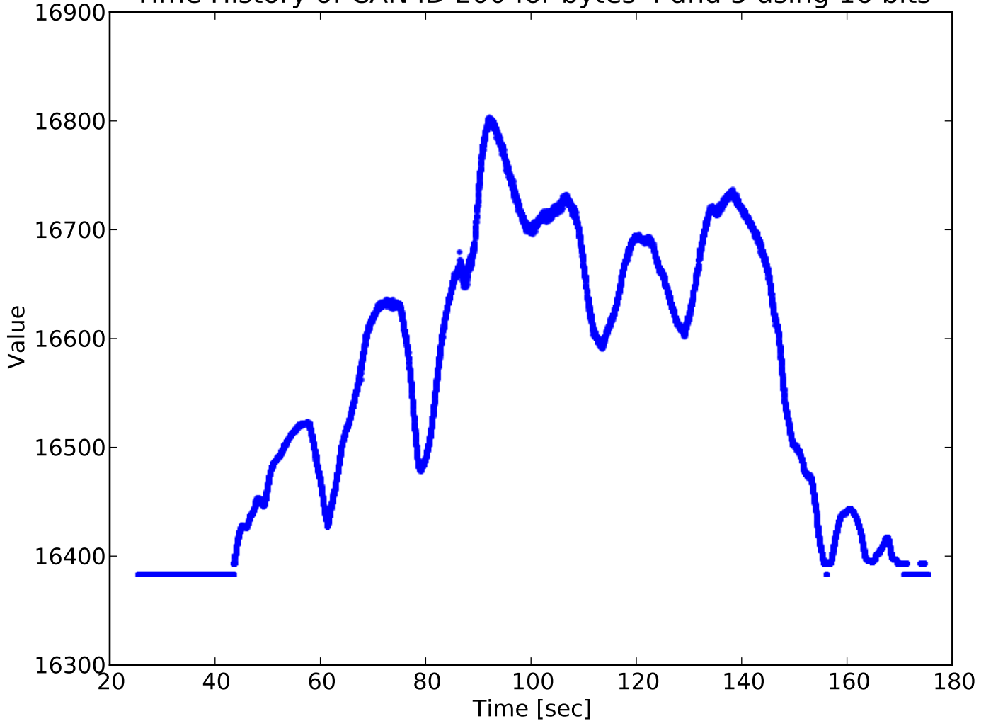
Time History of CAN ID 200 for bytes 4 and 5 using 16 bits
