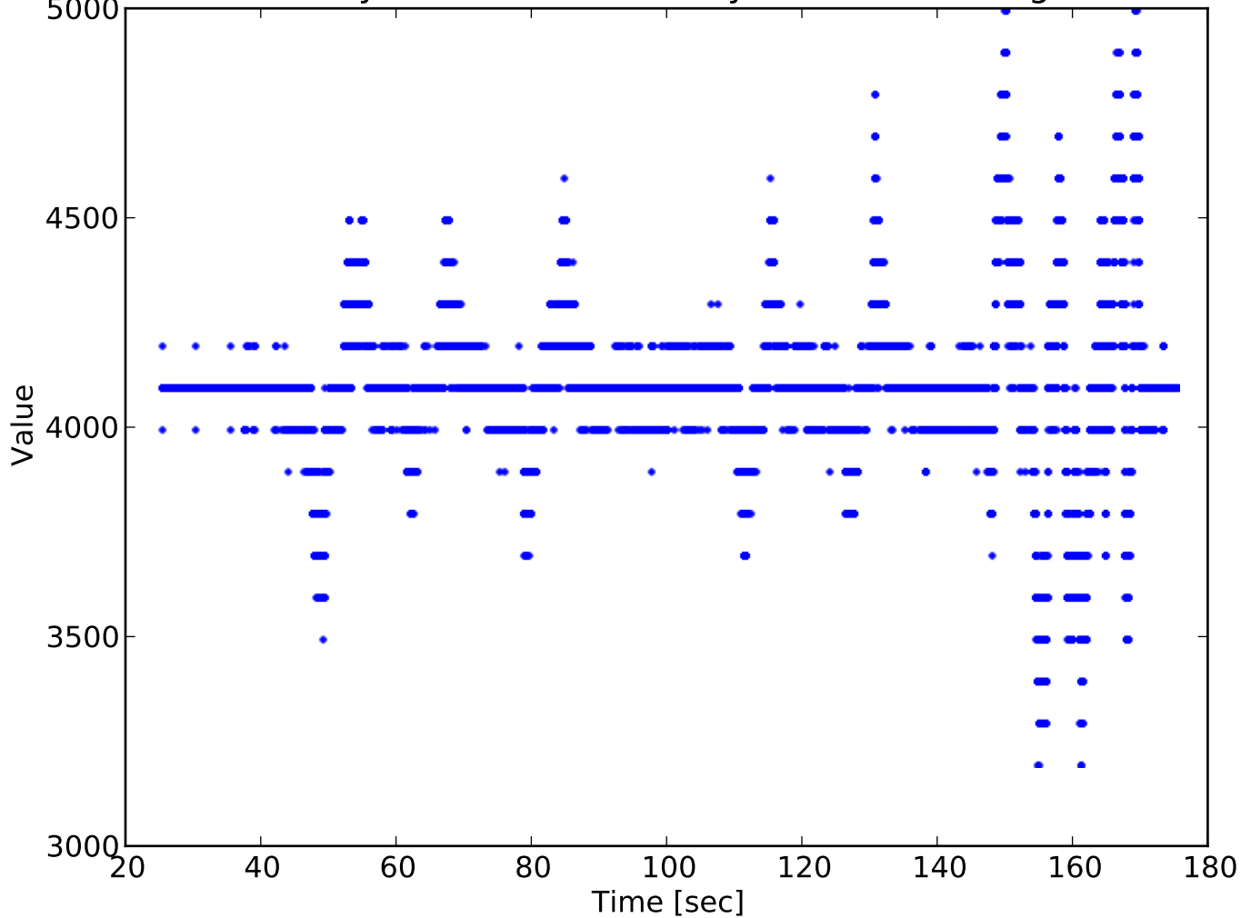
Time History of CAN ID 236 for bytes 2 and 3 using 16 bits
