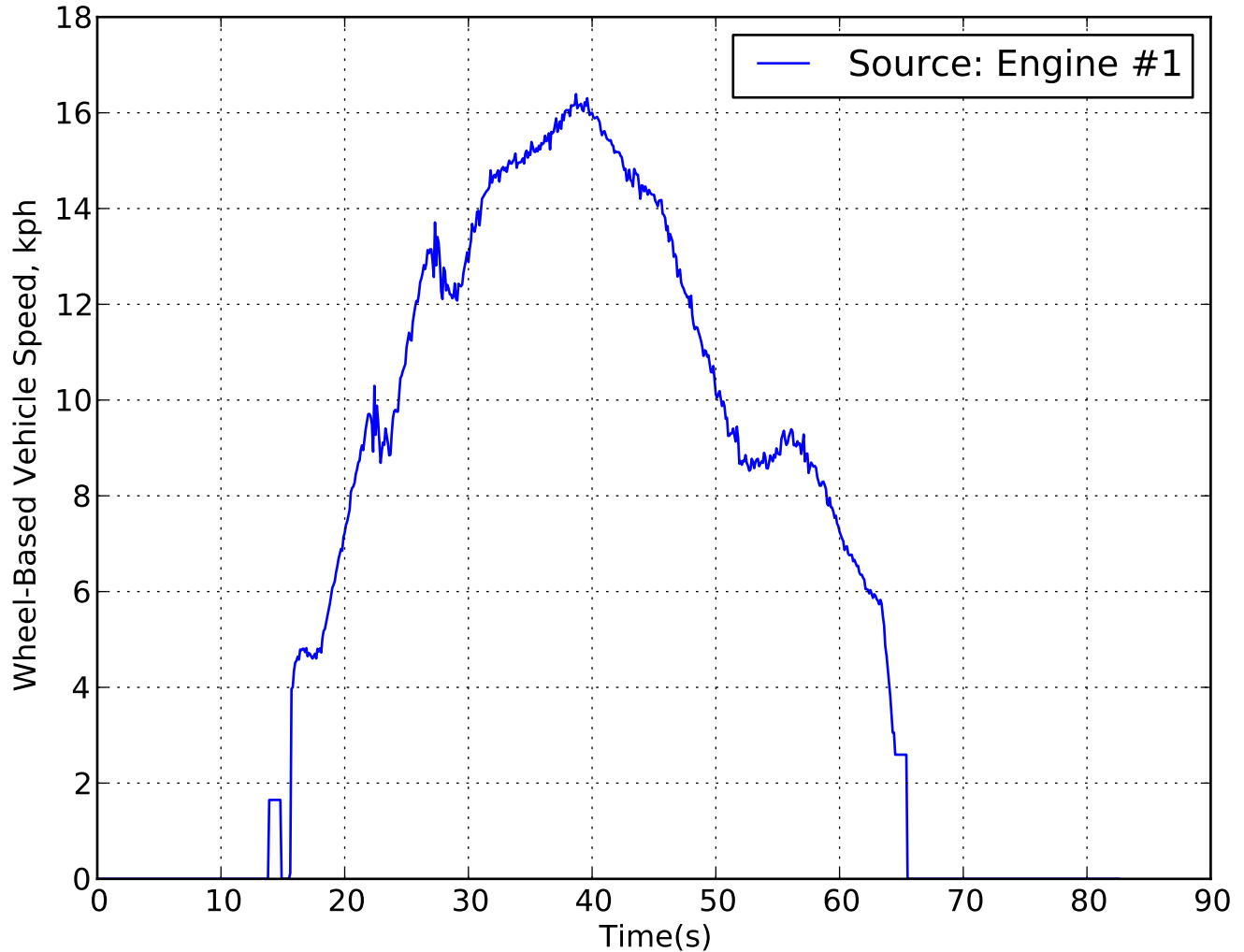
Data from RunData.db showing SPN 84 from the J1939 CCVS Message
